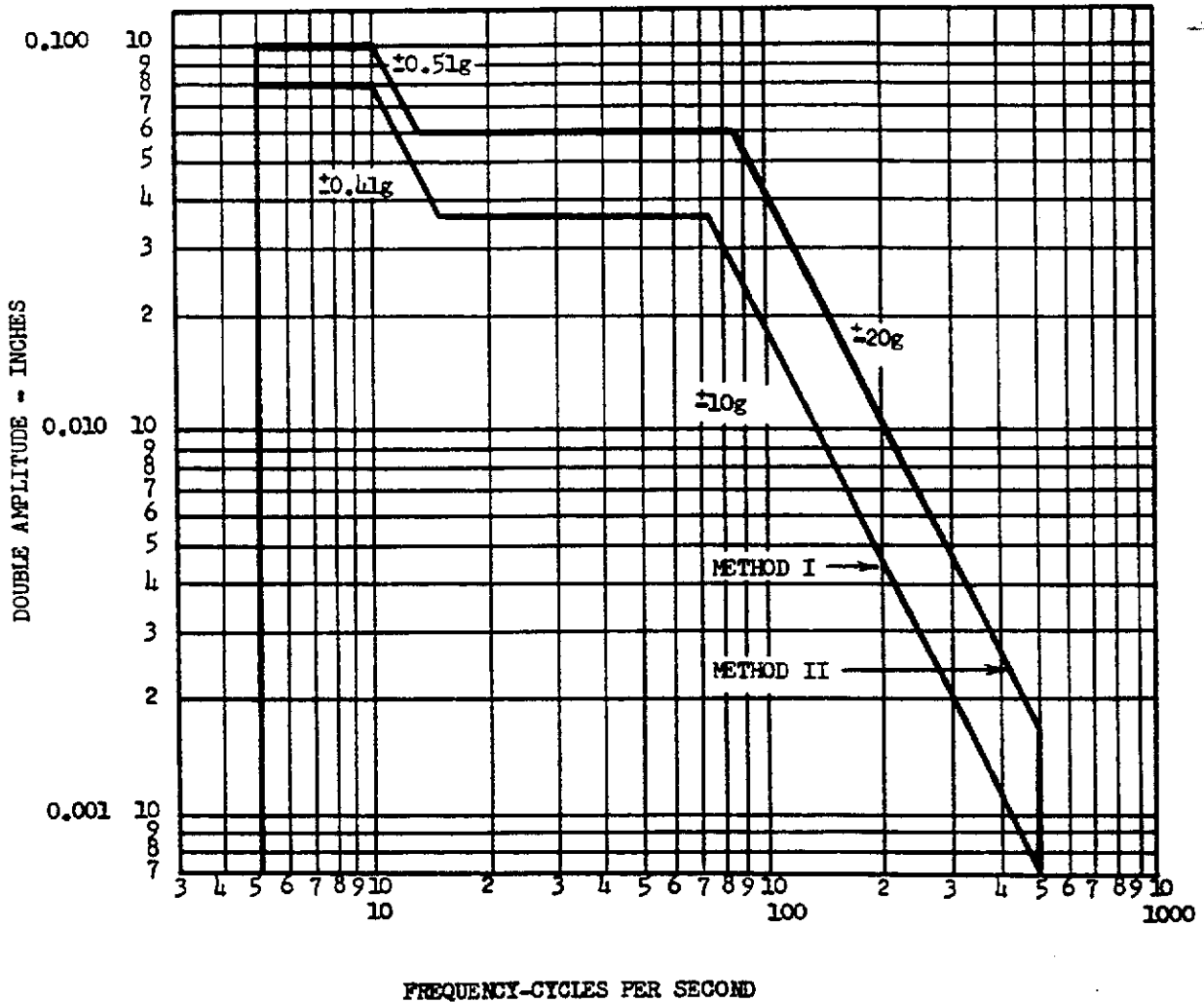
Figure 1.—Range curves for vibration tests.
