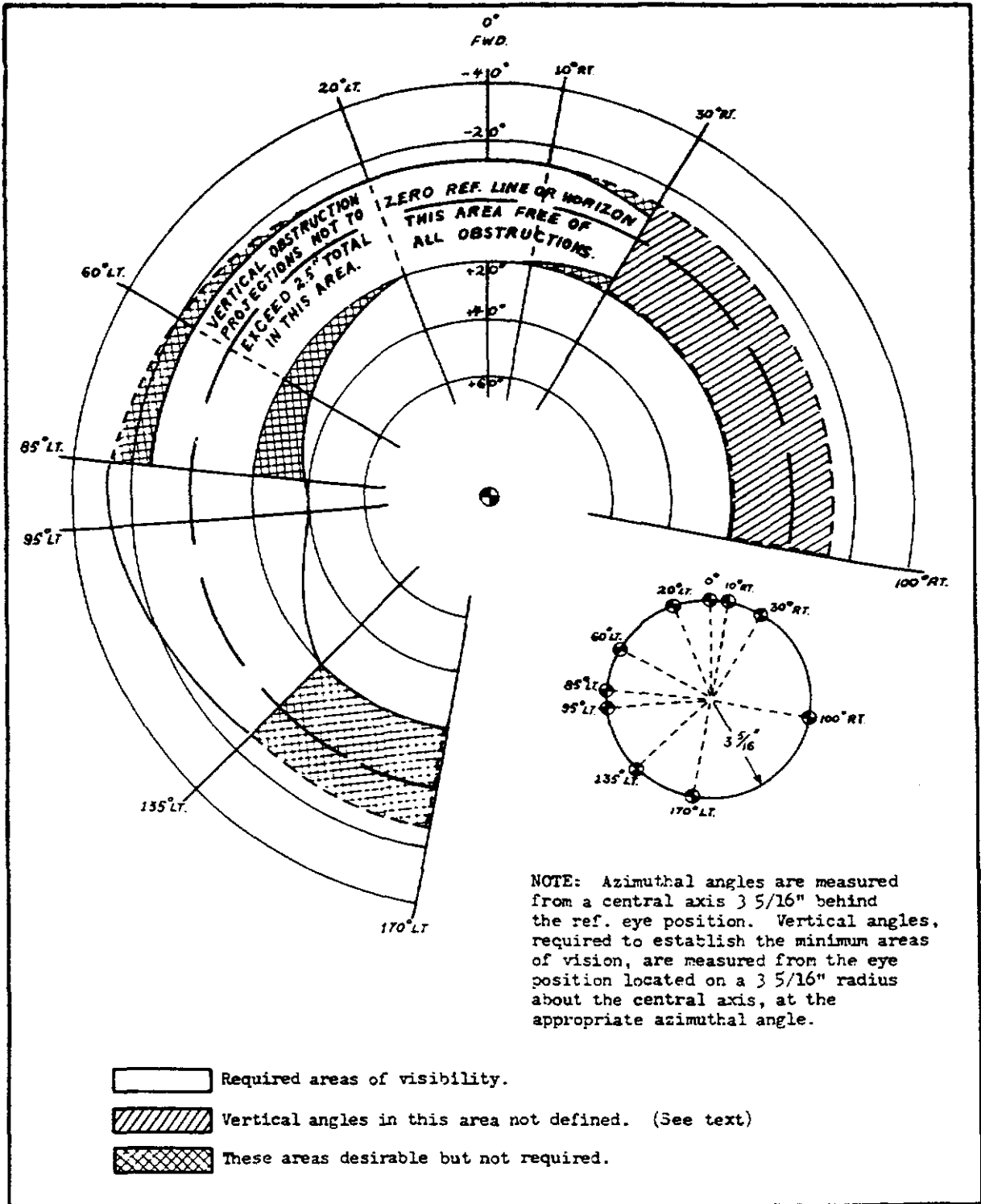
Figure 7.—Clear areas of vision.
