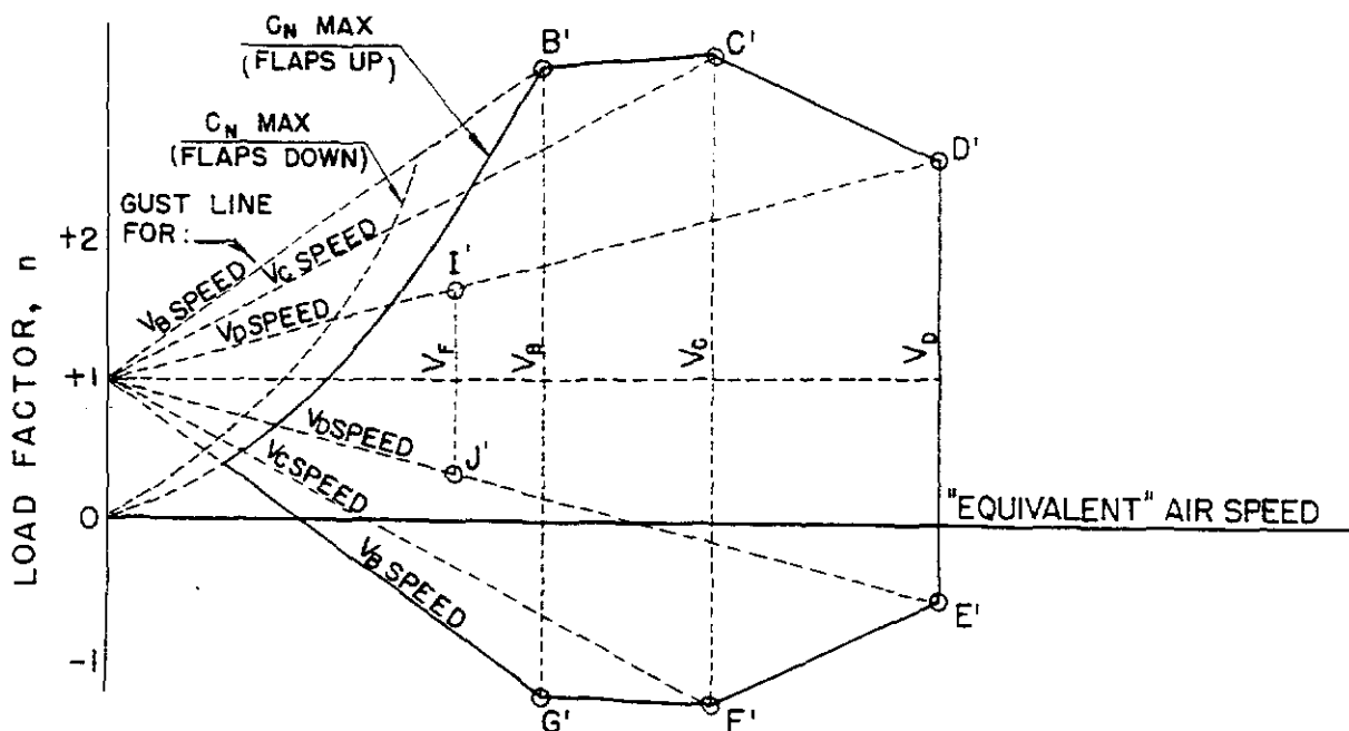
Figure 4b-3.—Gust envelope.
