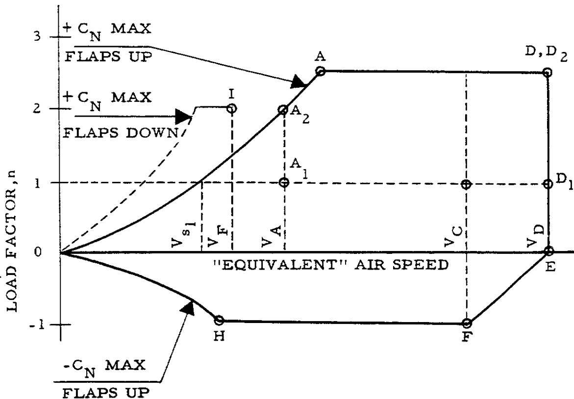
Figure 4b-2. —Maneuvering envelope.
