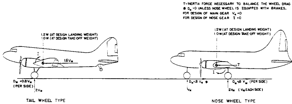
Figure 4b-12.—Braked roll.
