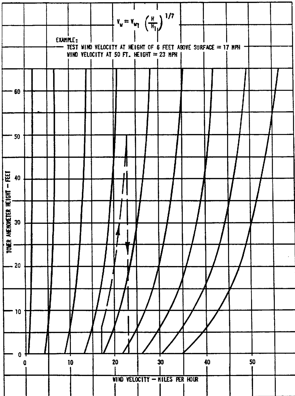
Figure 2. — Wind gradient correction.
