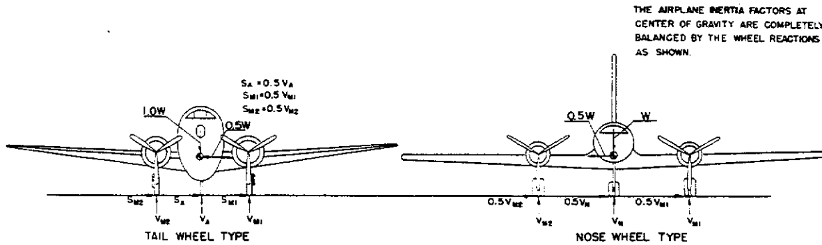
Figure 4b-13.—Ground turning.
