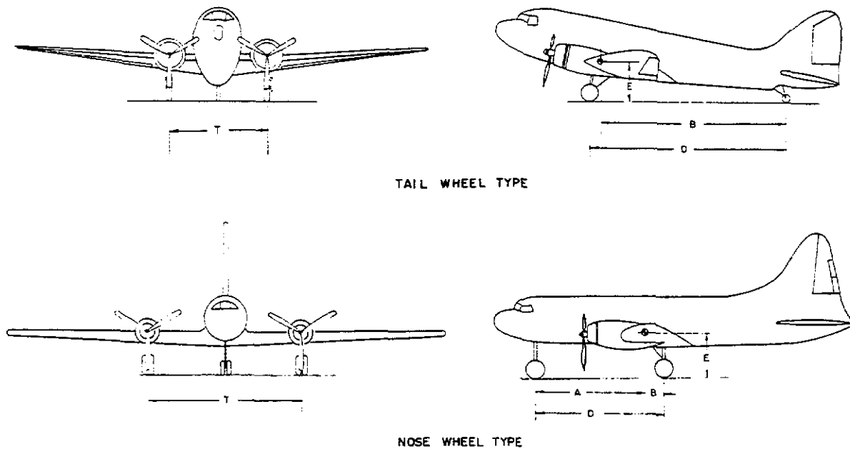
Figure 4b-7.—Basic landing gear dimension data.
